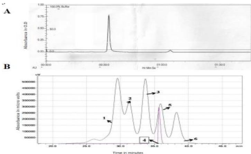
Figure 5: A: Purity analysis of rhGM-CSF protein by analytical size exclusion chromatography (SEC). Fifty micrograms of pure protein was loaded on Superdex 75™ column and eluted with phosphate buffer pH 7.2 with flow rate of 0.5 ml/min and displayed a single main peak. B: Size analysis of rhGM-CSF protein by size exclusion chromatography (SEC). Peak 1, 2, 3, 5 and 6 represent standard molecular weight markers as described in the methods. Peak 4 represent rhGM-CSF protein eluted between the peak 3 (29.0 kDa) and peak 5 (13.7 kDa) and size of conformed to 14.5 kDa.
