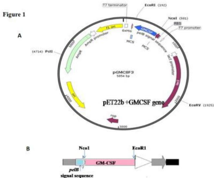
Figure 1: A. Construction of rhGM-CSF clone . Amplified hGM-CSF gene (384 bp) and pET-22b plasmid (5.4 kb) were digested with Nco I and Eco RI and hGM-CSF was ligated to upstream of T7 promoter next to pelB signal sequence. B. Physical map of part of the cassette of recombinant plasmid with signal sequence (pelB leader region) and hGM-CSF gene.
