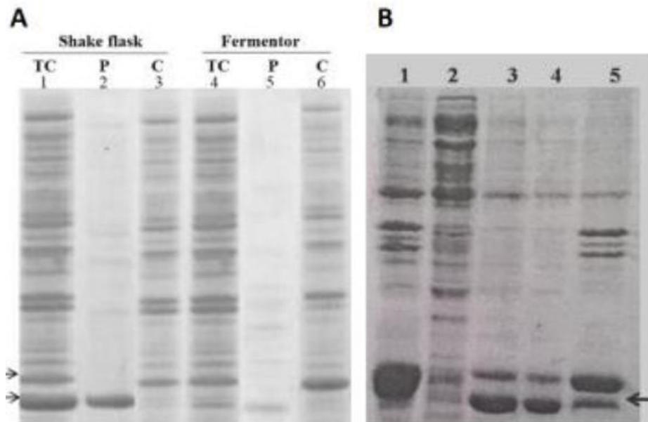
Figure 3: A: Subcellular localization of precursor and mature forms of GM-CSF by SDS-PAGE analysis. Total cellular, periplasmic and cytoplasmic extracts were isolated from E. coli shake flask and fermenter. The extracts were analysed on 14 % SDS-PAGE. Lane 1-3: Extractions from shake flask culture. Lane 4-6: Extractions from fermenter. TC: total cellular extracts, P: periplasmic extracts, C: cytoplasmic extracts. Arrows (top) indicates premature form (17 kDa) and bottom arrow indicated mature form (14.5 kDa) of rhGM-CSF. B. Analysis of samples after cell-lysis and solubilization at different time intervals samples were loaded on SDS-PAGE. Cell lysate was centrifuged at 12,000 rpm; pellet and supernatant were loaded on 14 % SDS-PAGE. The pellet was solubilized for 16 h and supernatant was subjected to SDS-PAGE at different time points. Lane 1, cell lysate pellet; lane 2, supernatant; lane 3, 4 and 5, are solubilized supernatant collected at 16, 8 and 0 h respectively. We observe that proportionately increased levels of mature rhGM-CSF with solubilization time. Arrow indicates the increased release of mature rhGM-CSF by in vitro signal peptidase action in presence of Triton X 100.
