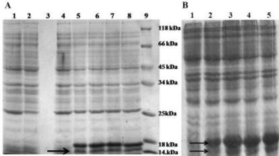
Figure 3: A: Subcellular localization of precursor and mature forms of GM-CSF by SDS-PAGE analysis. Total cellular, periplasmic and cytoplasmic extracts were isolated from E. coli shake flask and fermenter. The extracts were analysed on 14 % SDS-PAGE. Lane 1-3: Extractions from shake flask culture. Lane 4-6: Extractions from fermenter. TC: total cellular extracts, P: periplasmic extracts, C: cytoplasmic extracts. Arrows (top) indicates premature form (17 kDa) and bottom arrow indicated mature form (14.5 kDa) of rhGM-CSF. B. Analysis of samples after cell-lysis and solubilization at different time intervals samples were loaded on SDS-PAGE. Cell lysate was centrifuged at 12,000 rpm; pellet and supernatant were loaded on 14 % SDS-PAGE. The pellet was solubilized for 16 h and supernatant was subjected to SDS-PAGE at different time points. Lane 1, cell lysate pellet; lane 2, supernatant; lane 3, 4 and 5, are solubilized supernatant collected at 16, 8 and 0 h respectively. We observe that proportionately increased levels of mature rhGM-CSF with solubilization time. Arrow indicates the increased release of mature rhGM-CSF by in vitro signal peptidase action in presence of Triton X 100.
