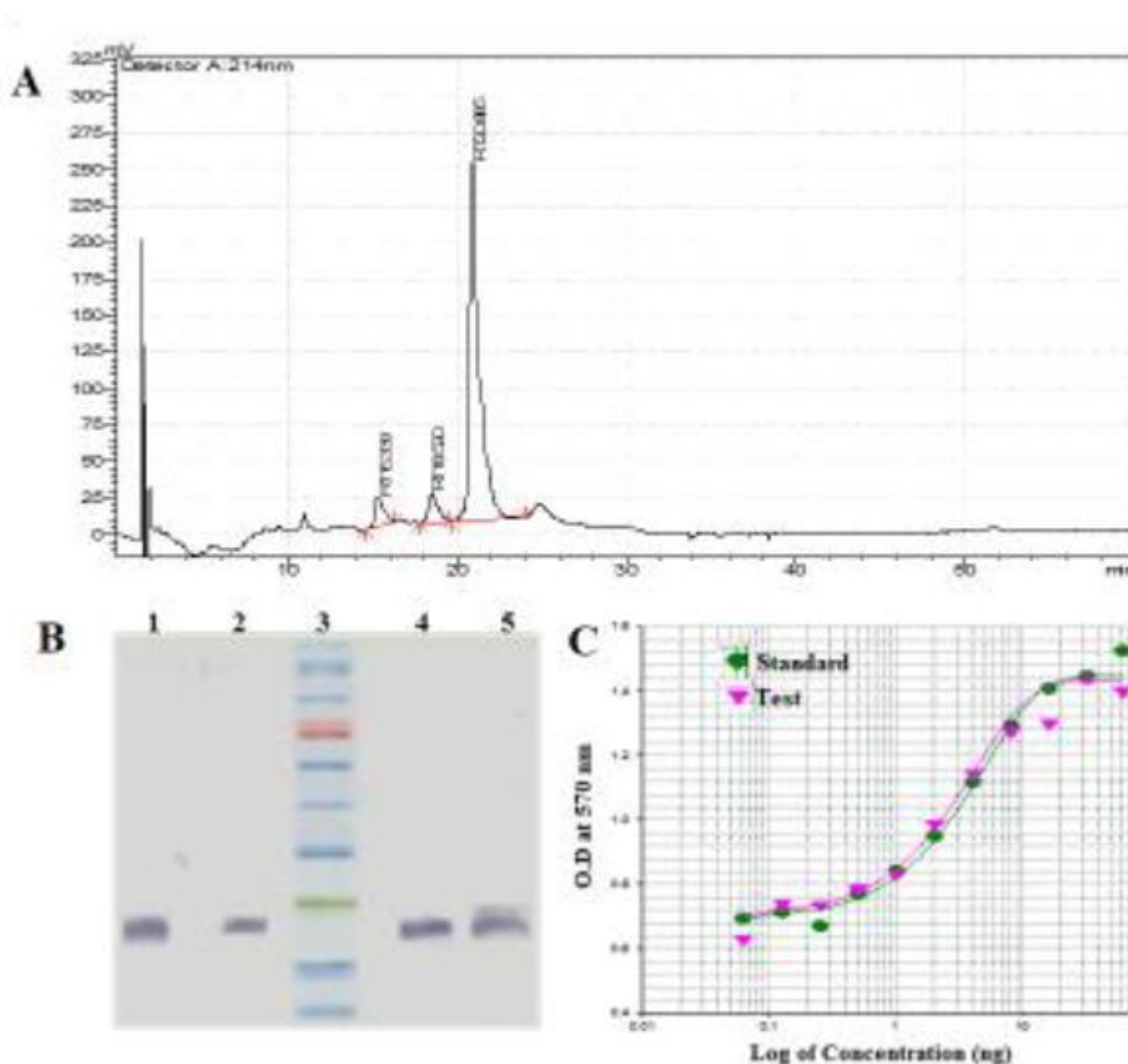
Fig 6 A: Reversed phase chromatography (RPC) analysis of purified rhGM-CSF. Final protein was loaded on the RPC column and percentage of each peak was analyzed. Peak 3 represent the rhGM-CSF and show more than 98 % pure and the remaining minor peaks are impurities represent less than 1.5 %. B: Immunoblot analysis of rhGM-CSF protein. Both standard and test protein samples were loaded on SDS-PAGE and transferred on PVDF membrane and probed with anti-GM-CSF antibody as described in the methods. Lanes 1 and 5, standard and test samples were run under non-reducing conditions respectively; lane 2 and 4, standard and test samples were run under reducing conditions. C: Cell proliferation assay. Ability of rhGM-CSF purified protein biological activity on cell proliferation was assessed against a NIBSC reference standard as described in methods. Color product was measured spectrophotometrically and obtained data was analyzed by fitting a sigmoidal dose response curves. The data in this figure is a representative of three different batches run in triplicates. Circles indicate NIBSC reference standard, triangles indicate purified rhGM-CSF.
